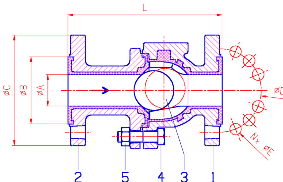
Dimensional Chart B201 (DIN version)
